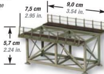
Vorfluter-Brücke (ohne Brückenköpfe) Truss Approach Bridge (without bridge heads)
